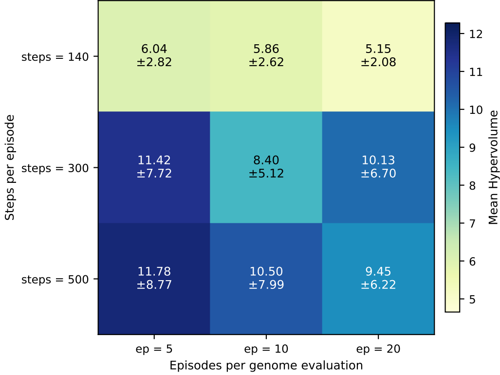
Figure 2: Scale sensitivity heatmap: mean HV by simulation horizon (steps \times episodes/genome). Each cell is n=10 independent NSGA-II runs. HV generally increases with steps; non-monotonicities between the 300- and 500-step rows reflect high between-run variance. Episode count has a weaker secondary effect.
